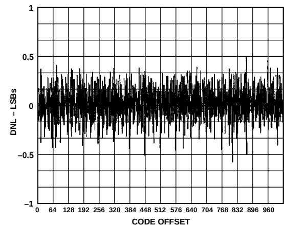
Figure 3. AD876 Typical DNL
